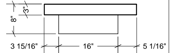
3 SIDE ELEV - COUNTERTOP SCALE 3/4" = 1'-0"
