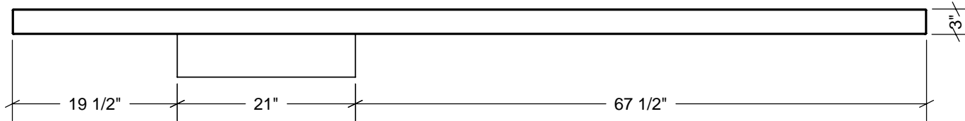
2 FRONT ELEV - COUNTERTOP SCALE 3/4" = 1'-0"
