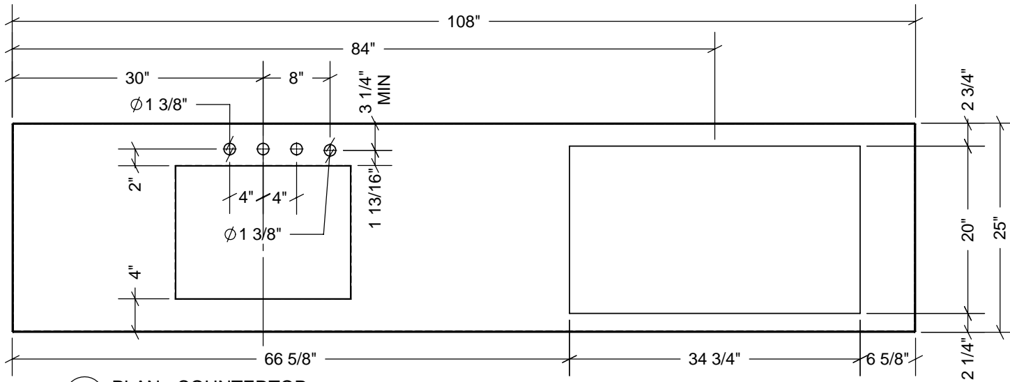
1 PLAN - COUNTERTOP SCALE 3/4" = 1'-0"
